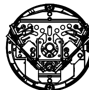
Top View LED Lumilock Assembly
